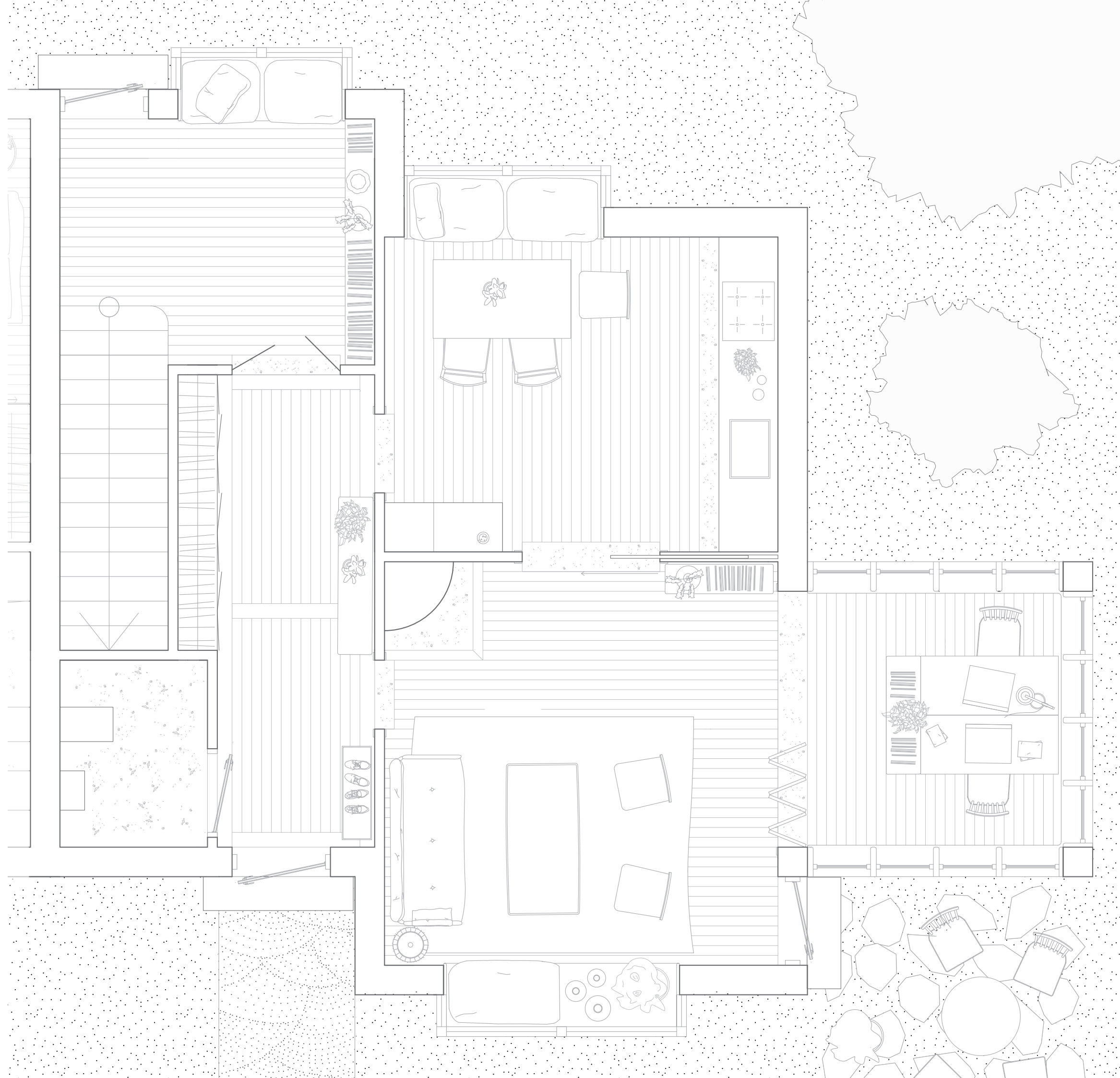
First floor of two-story home Option 1 1:25
