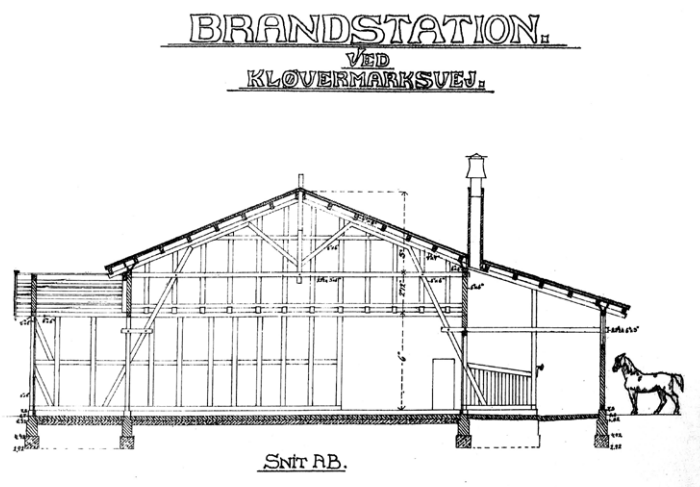
Snittegning, Christianshavns Brandstation, 1904
